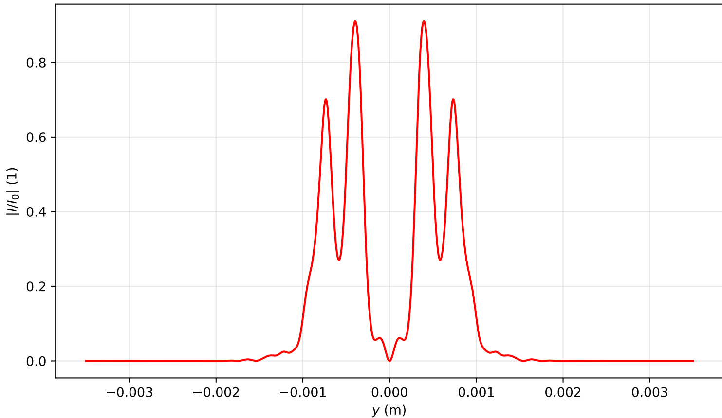
Intensity profile I(x=0, y, z=0.557)/I_0 , P_{in}=18.0\text{Pcr} , artificial time
