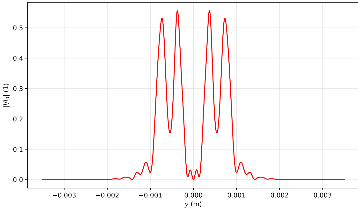
Intensity profile I(x=0, y, z=0.637)/I_0 , P_{in}=18.0\text{Pcr} , artificial time
