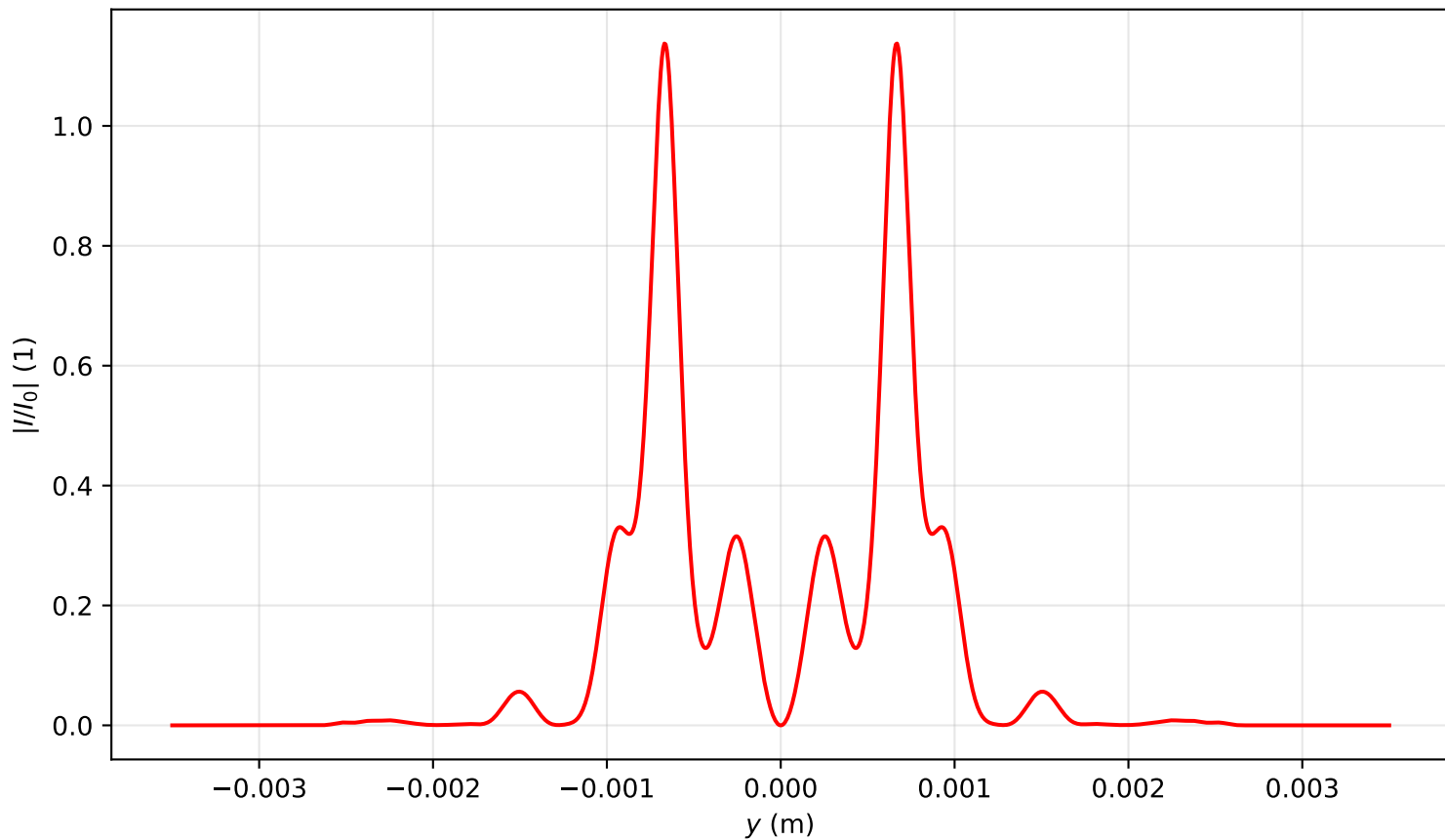
Intensity profile I(x=0, y, z=1.035)/I_0 , P_{in}=18.0P_{cr} , artificial time
