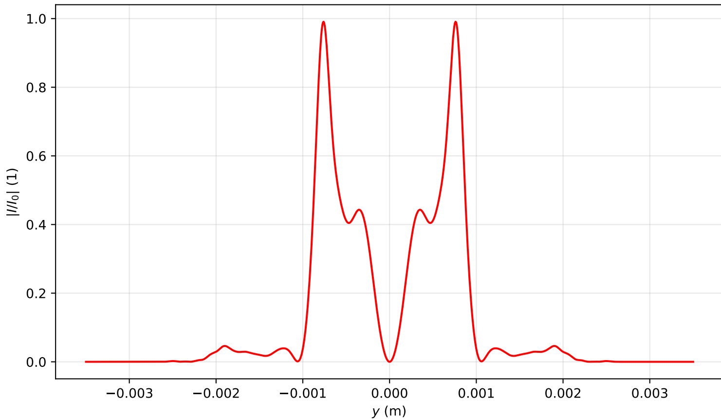
Intensity profile I(x=0, y, z=1.274)/I_0 , Pin=18.0Pcr, artificial time
