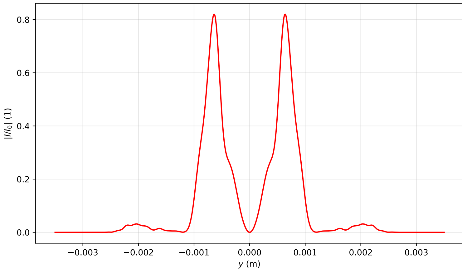
Intensity profile I(x=0, y, z=1.353)/I_0 , P_{in}=18.0P_{cr} , artificial time
