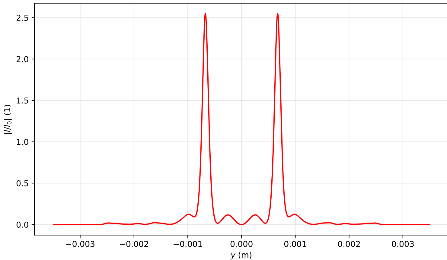
Intensity profile I(x=0, y, z=1.513)/I_0 , P_{in}=18.0P_{cr} , artificial time
