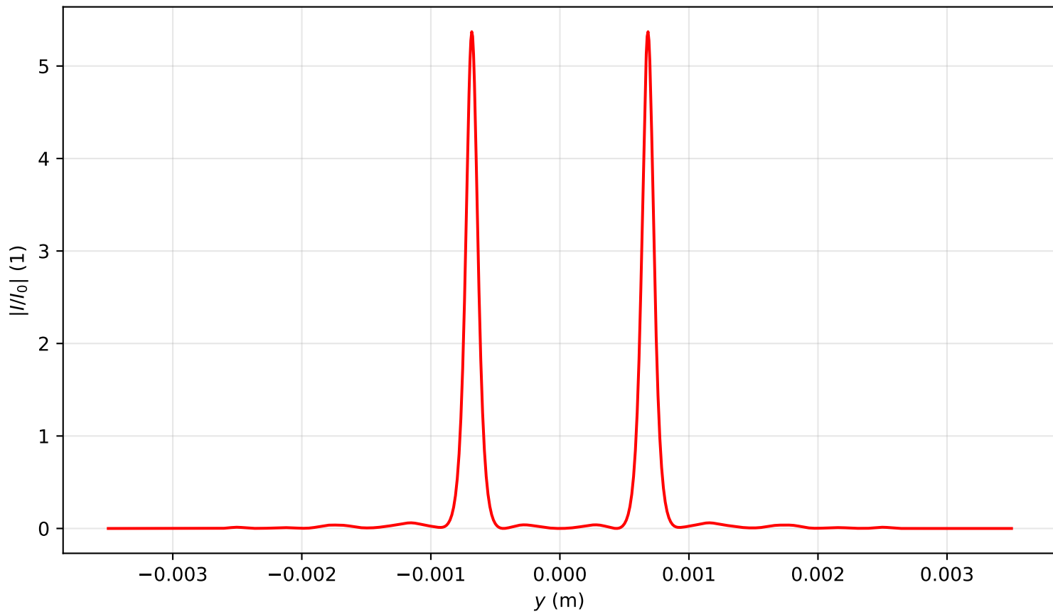
Intensity profile I(x = 0, y, z = 1.592)/I_0 , P_{in}=18.0\text{Pcr} , artificial time
