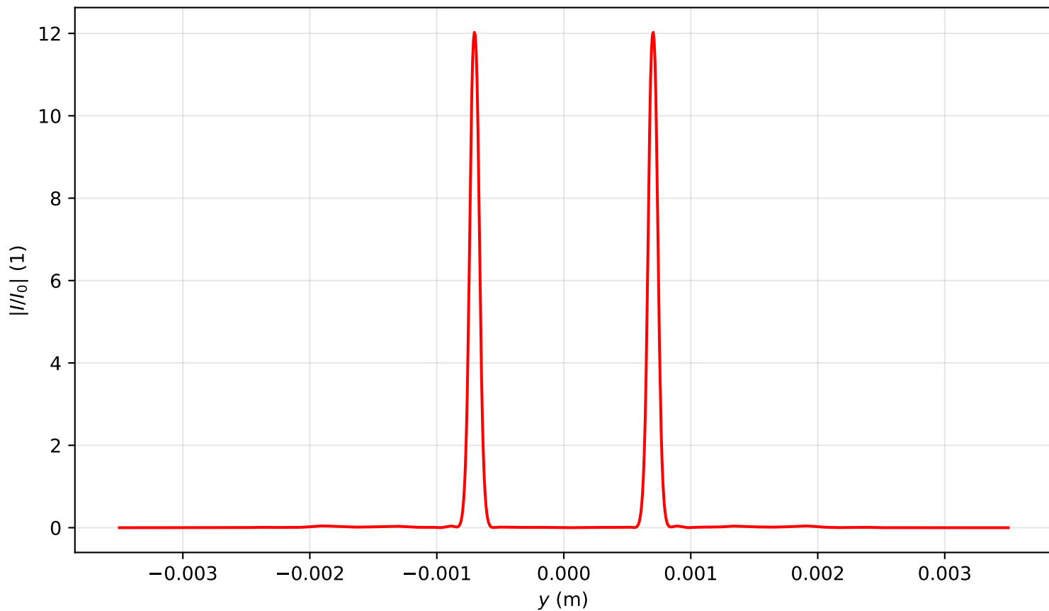
Intensity profile I(x = 0, y, z = 1.672)/I_0 , \text{Pin}=18.0\text{Pcr} , artificial time
