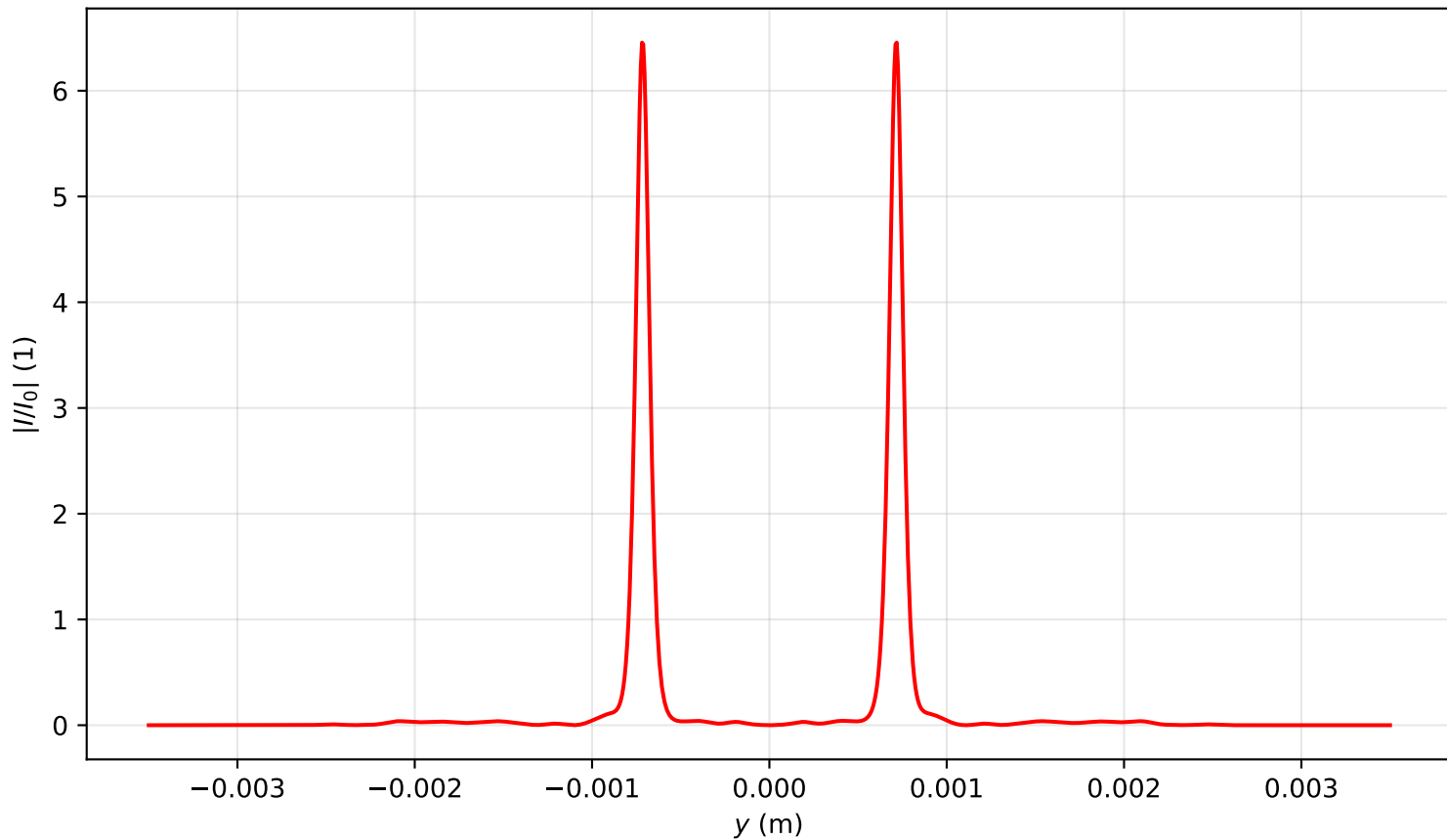
Intensity profile I(x=0, y, z=1.751)/I_0 , P_{in}=18.0\text{Pcr} , artificial time
