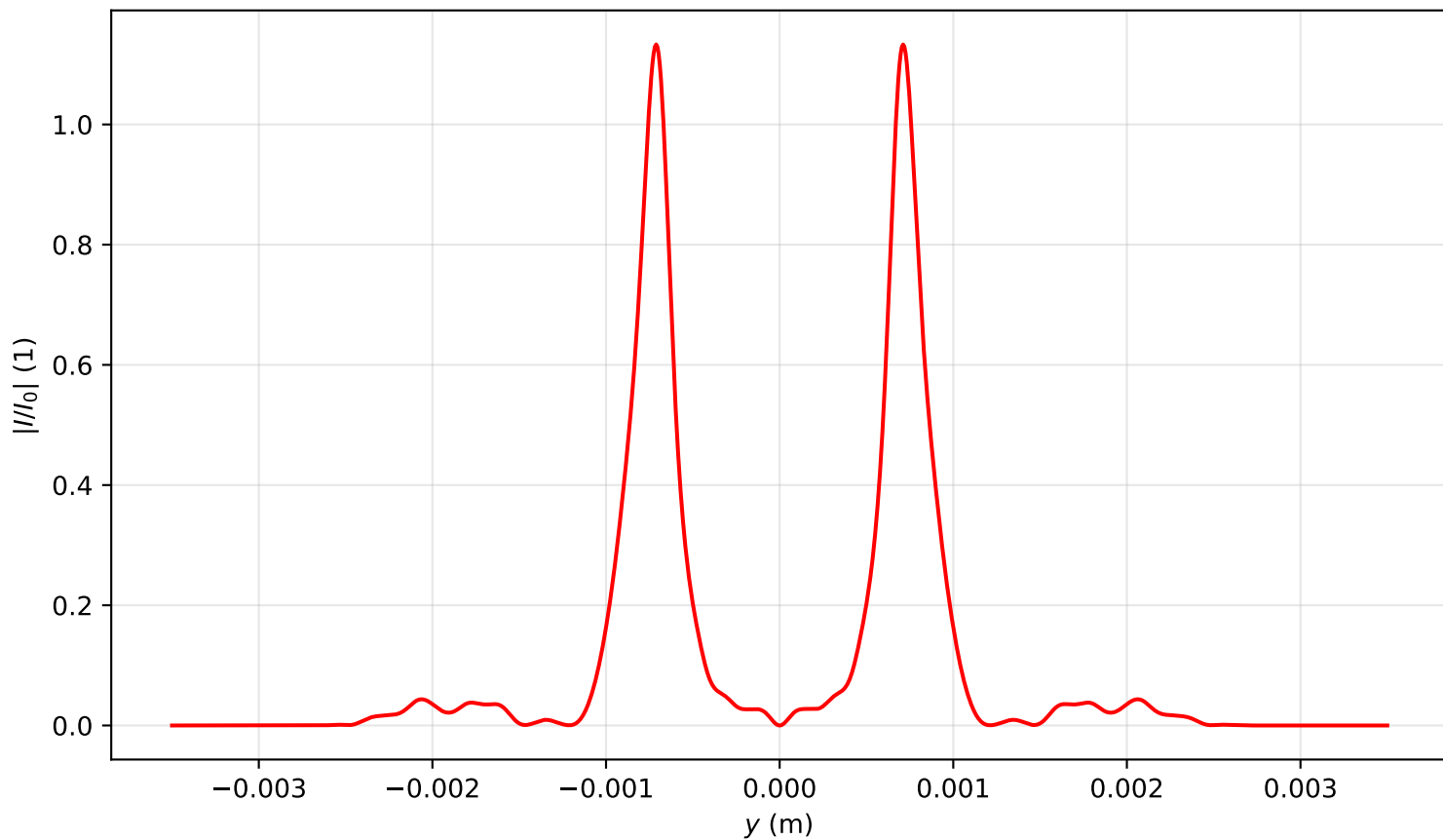
Intensity profile I(x=0, y, z=1.831)/I_0 , P_{in}=18.0\text{Pcr} , artificial time
