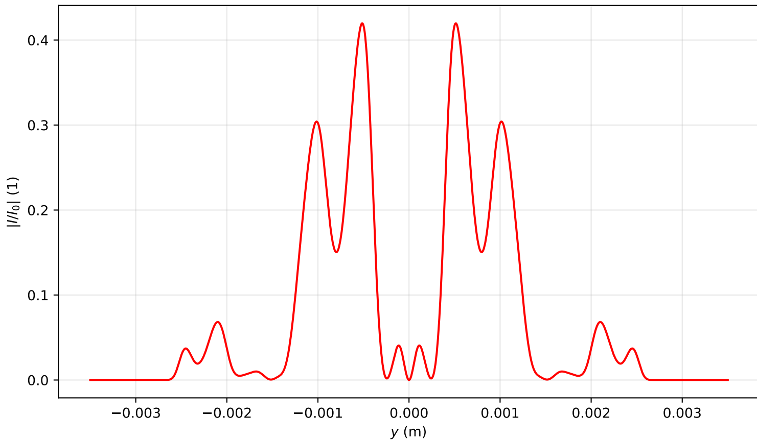
Intensity profile I(x=0, y, z=2.070)/I_0 , P_{in}=18.0P_{cr} , artificial time
