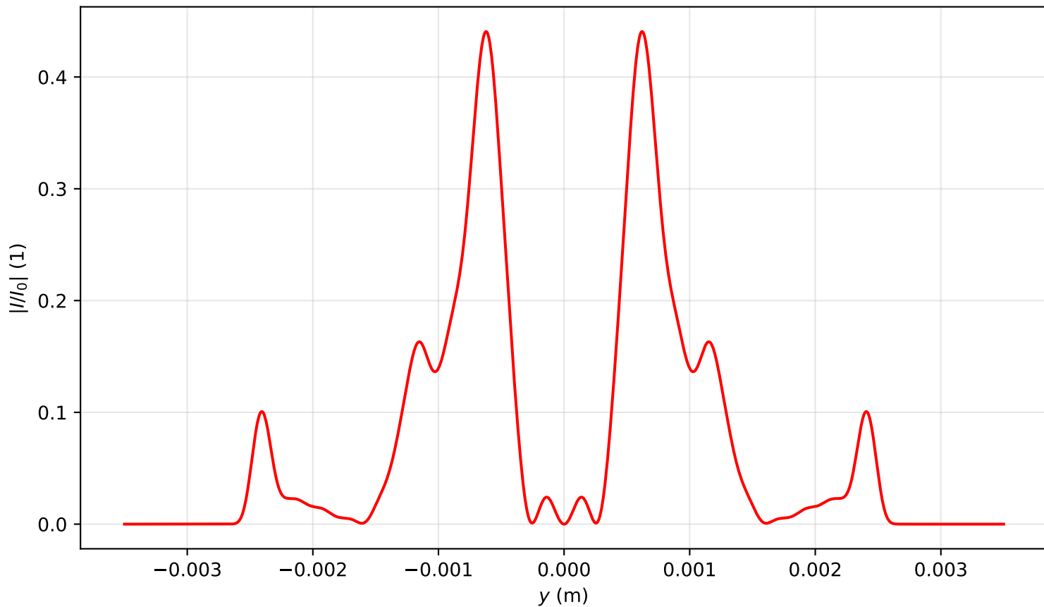
Intensity profile I(x=0, y, z=2.229)/I_0 , P_{in}=18.0\text{Pcr} , artificial time
