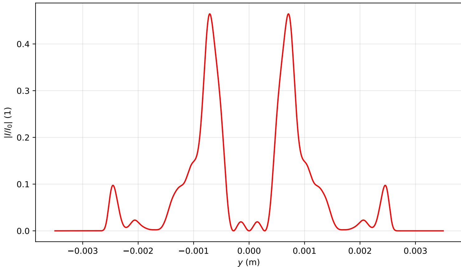
Intensity profile I(x=0, y, z=2.309)/I_0 , P_{in}=18.0\text{Pcr} , artificial time
