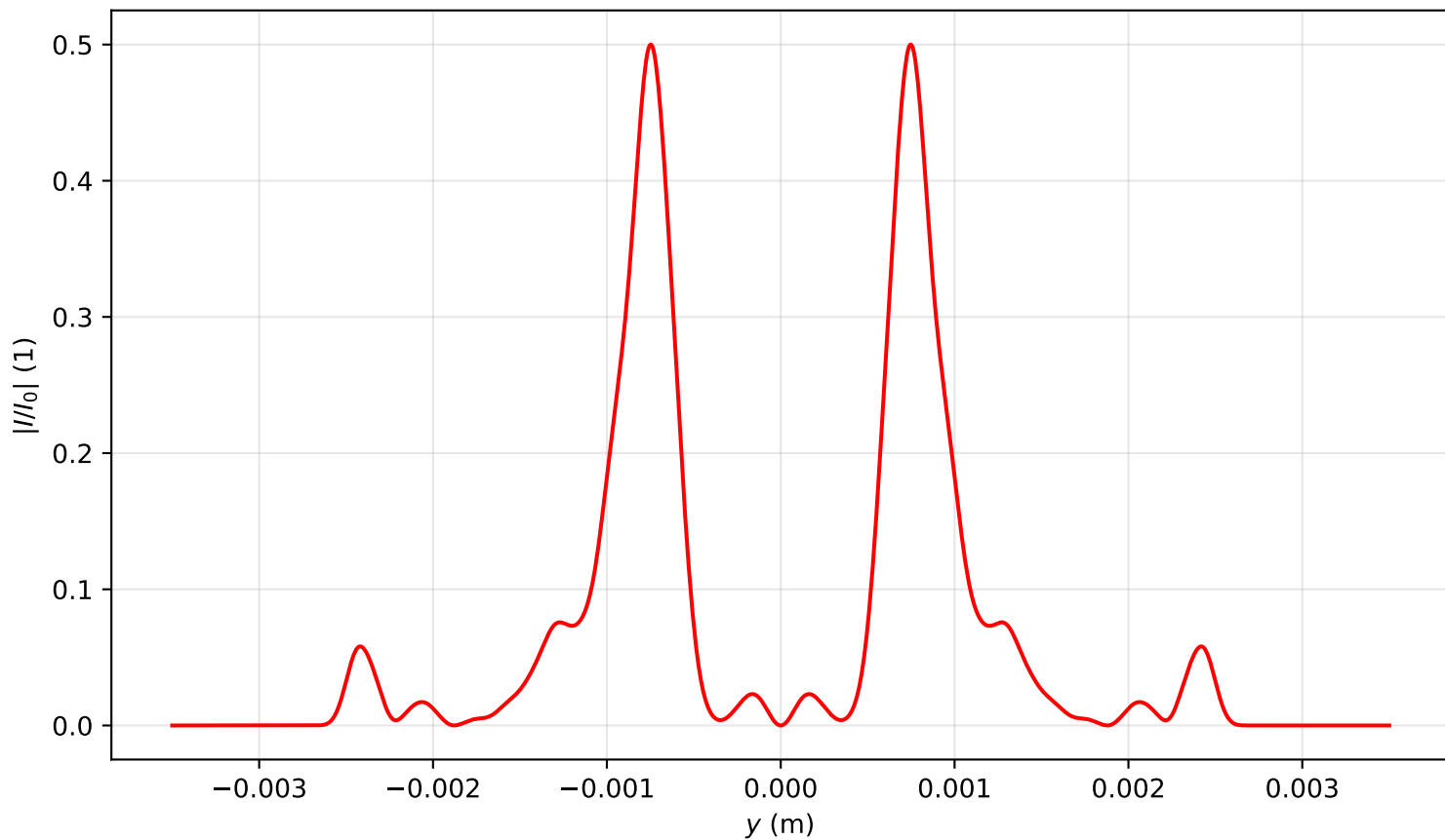
Intensity profile I(x=0, y, z=2.468)/I_0 , P_{in}=18.0\text{Pcr} , artificial time
