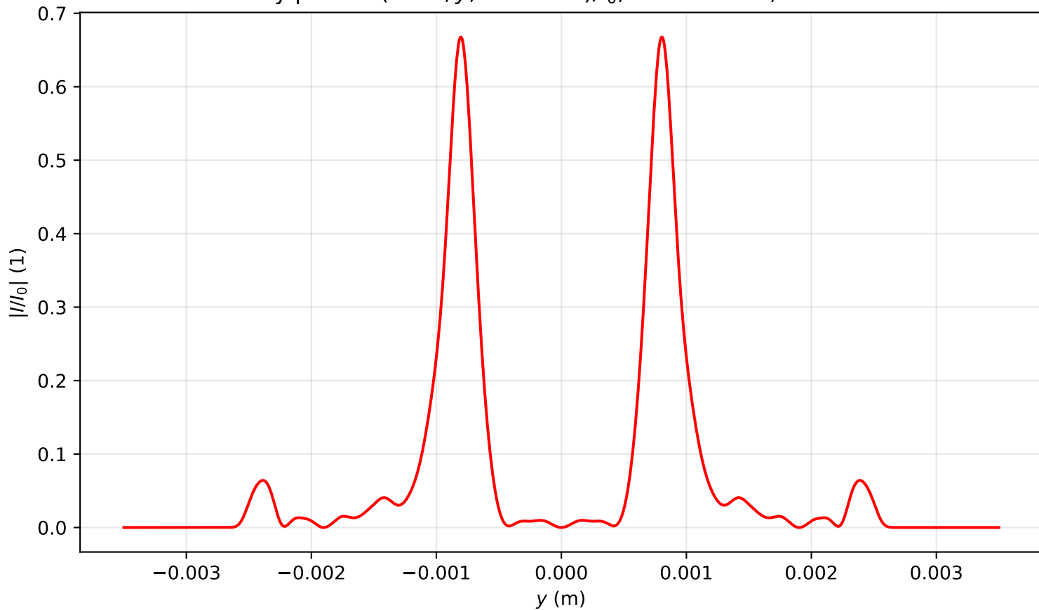
Intensity profile I(x=0, y, z=2.548)/I_0 , P_{in}=18.0\text{Pcr} , artificial time
