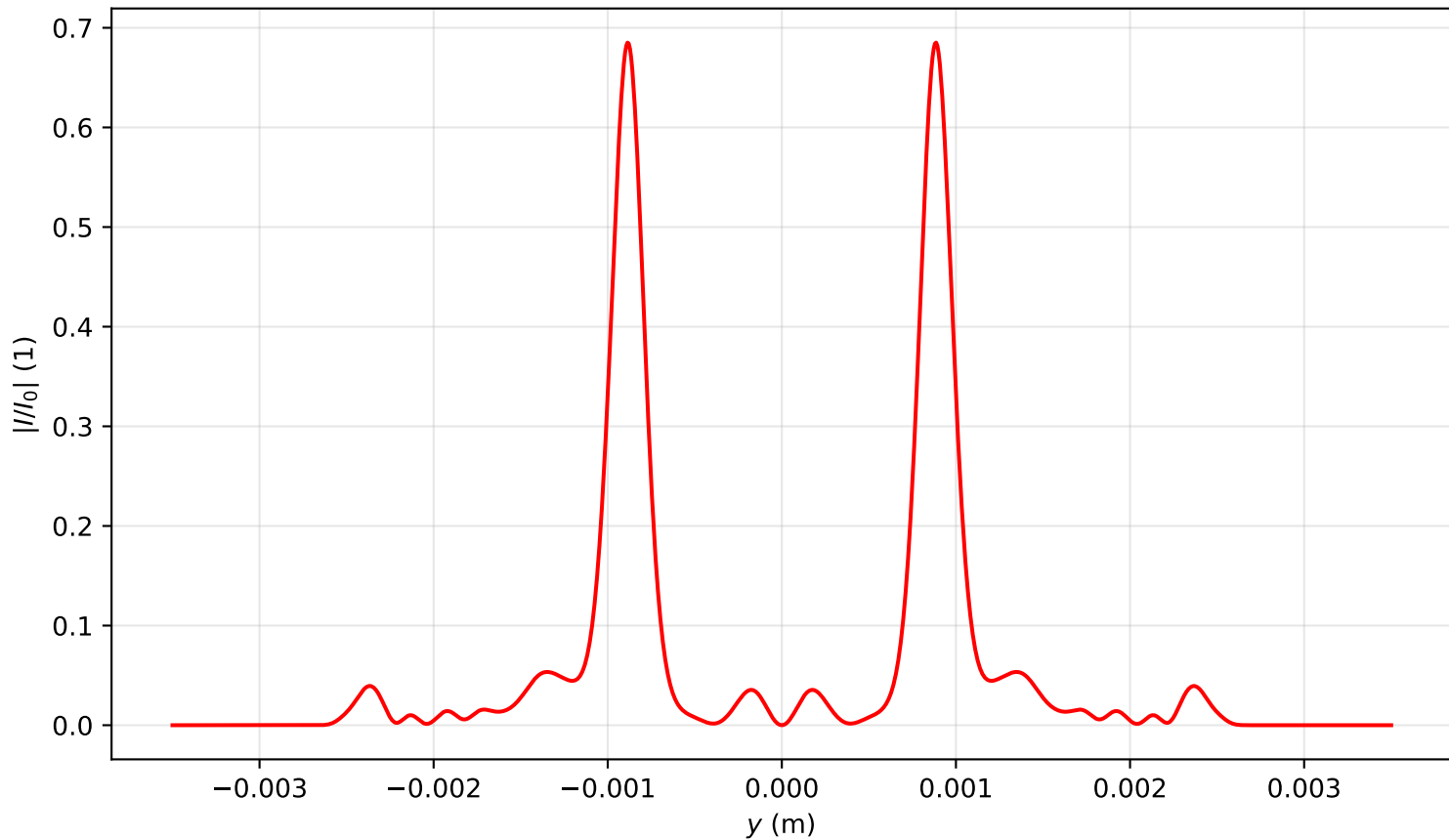
Intensity profile I(x=0, y, z=2.707)/I_0 , P_{in}=18.0P_{cr} , artificial time
