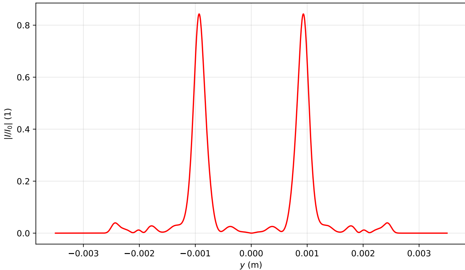
Intensity profile I(x=0, y, z=2.786)/I_0 , P_{in}=18.0\text{Pcr} , artificial time
