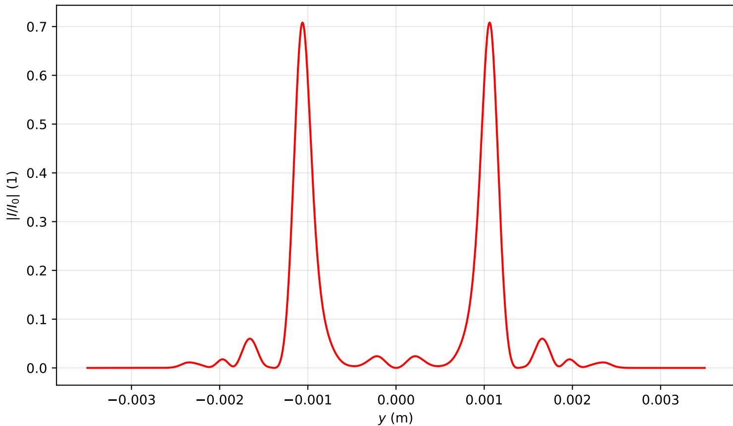
Intensity profile I(x=0, y, z=3.025)/I_0 , P_{in}=18.0\text{Pcr} , artificial time
