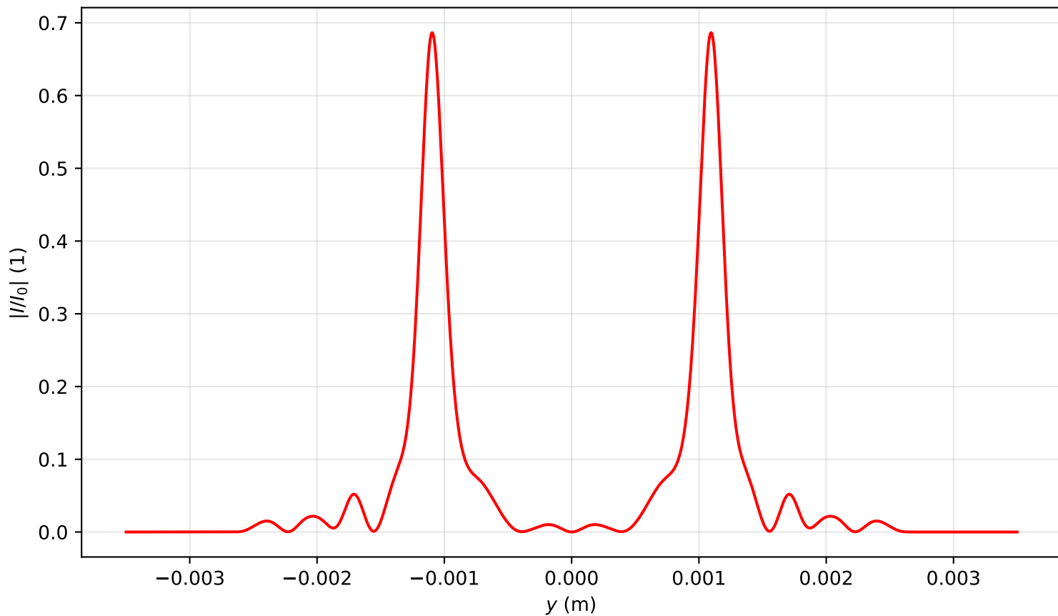
Intensity profile I(x=0, y, z=3.184)/I_0 , P_{in}=18.0P_{cr} , artificial time
