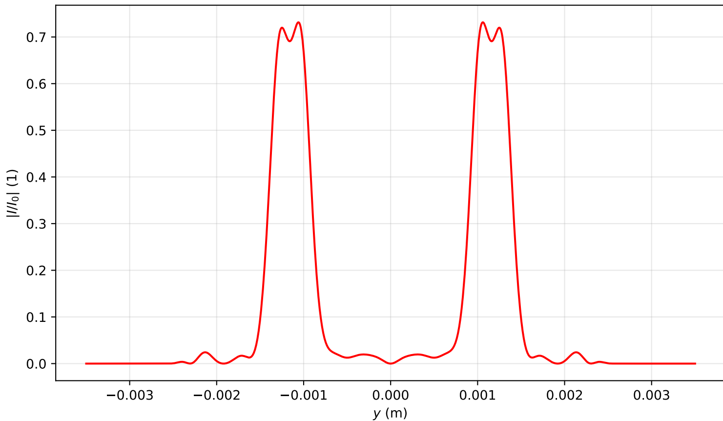
Intensity profile I(x=0, y, z=3.423)/I_0 , P_{in}=18.0P_{cr} , artificial time
