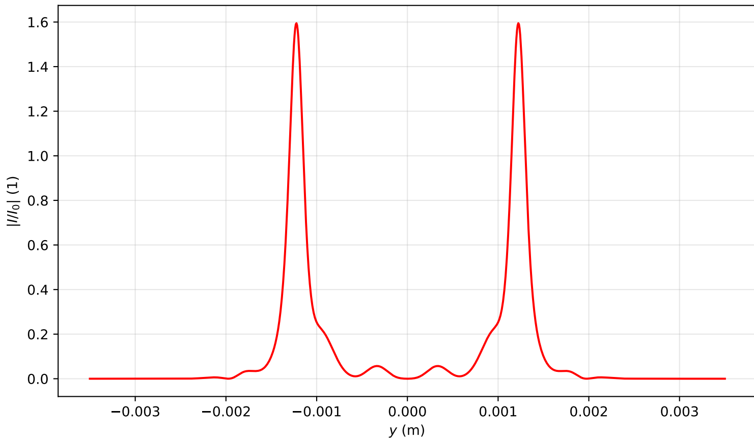
Intensity profile I(x=0, y, z=3.662)/I_0 , P_{in}=18.0P_{cr} , artificial time
