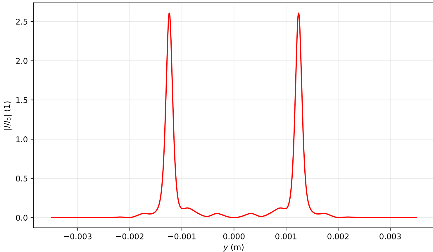
Intensity profile I(x=0, y, z=3.742)/I_0 , P_{in}=18.0P_{cr} , artificial time
