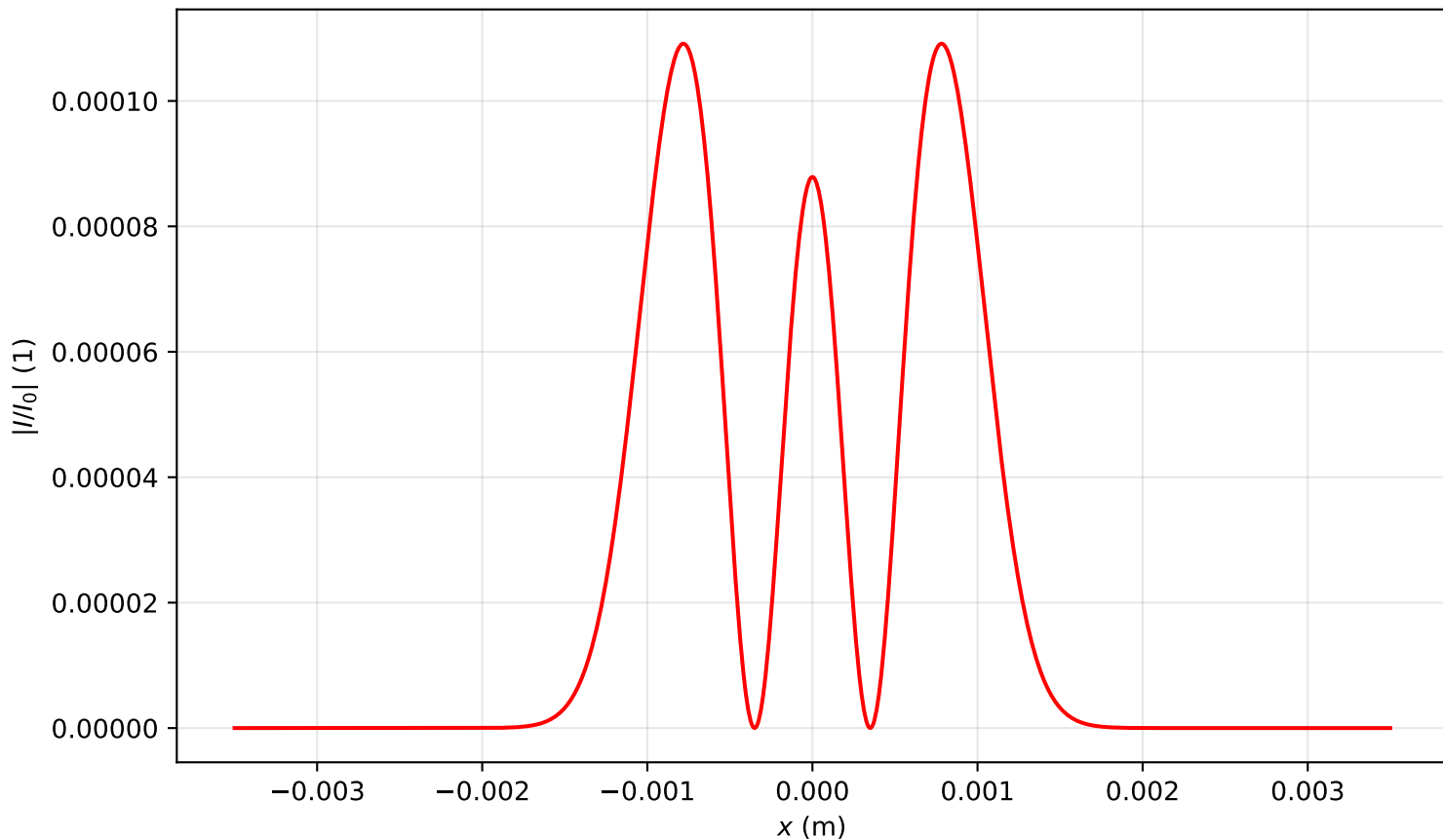
Intensity profile I(x, y = 0, z = 0.080)/I_0 , P_{in}=19.0P_{cr} , artificial time
