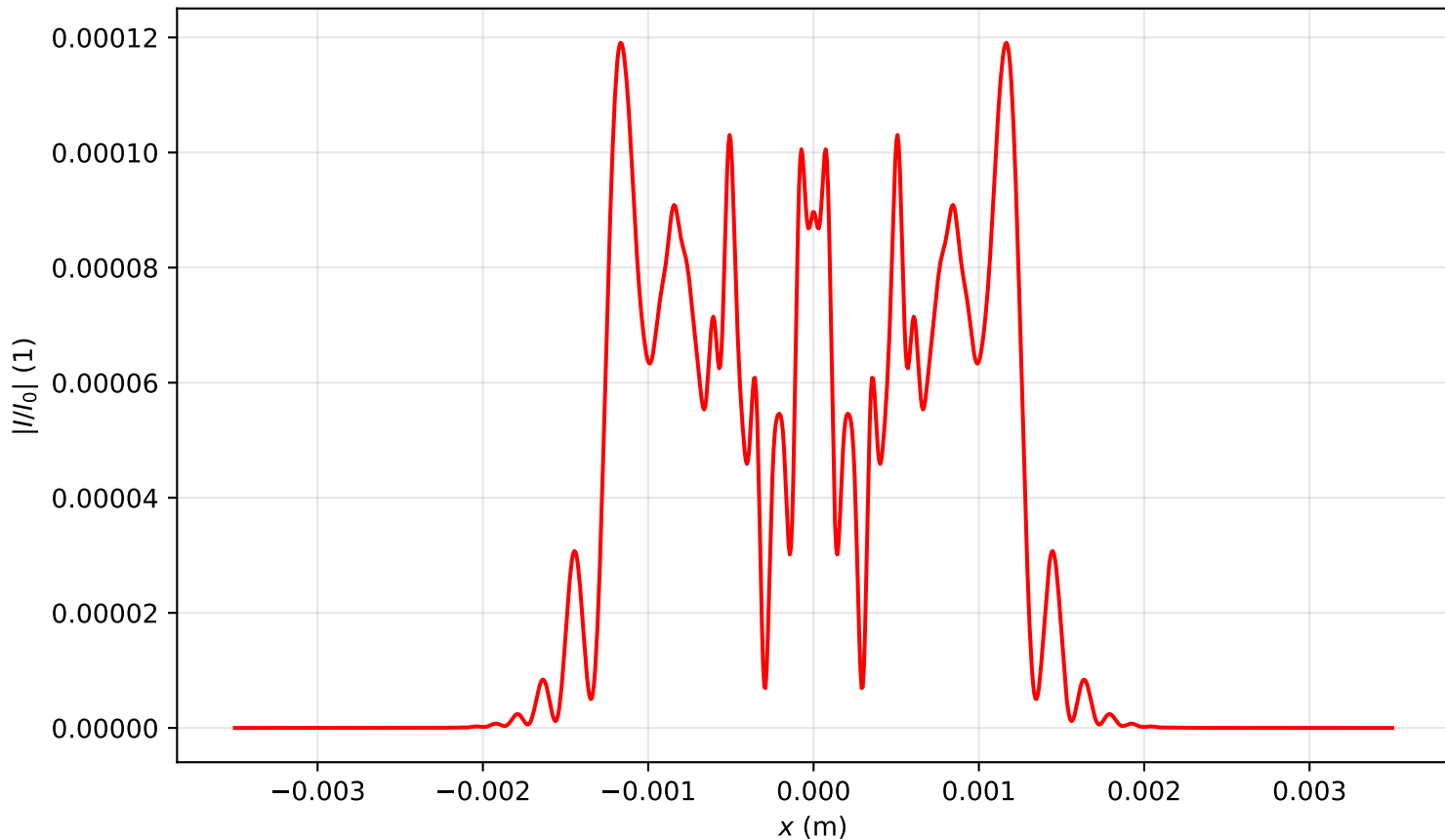
Intensity profile I(x, y = 0, z = 0.398)/I_0 , P_{in}=19.0P_{cr} , artificial time
