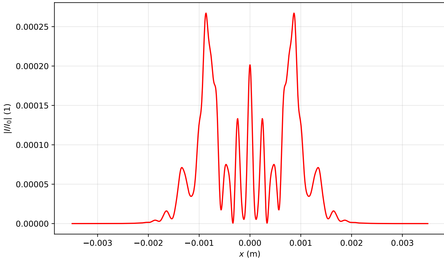
Intensity profile I(x, y = 0, z = 0.478)/I_0 , P_{in}=19.0P_{cr} , artificial time
