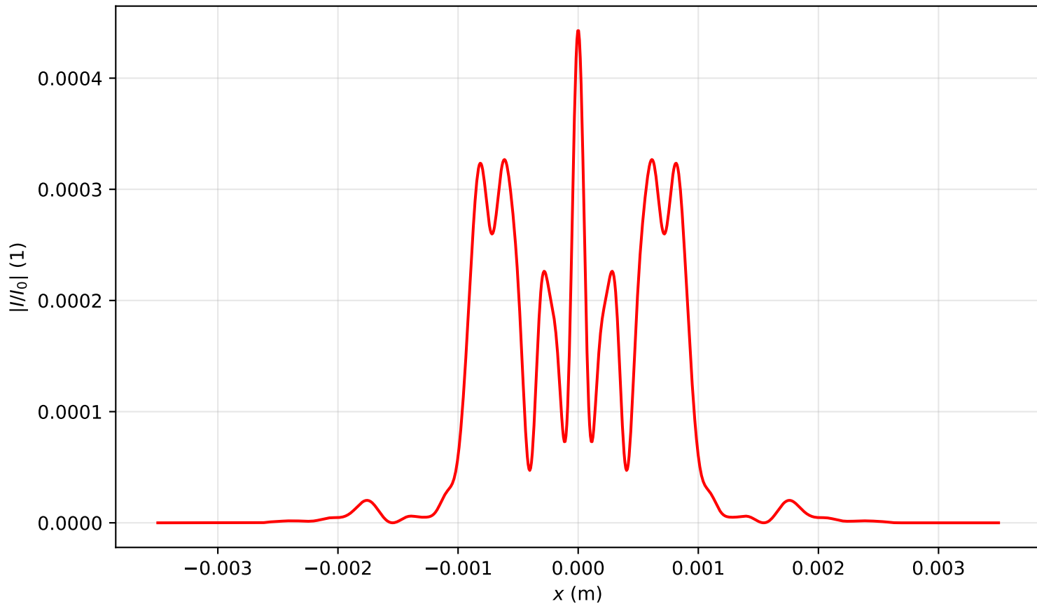
Intensity profile I(x, y = 0, z = 0.716)/I_0 , P_{in}=19.0P_{cr} , artificial time
