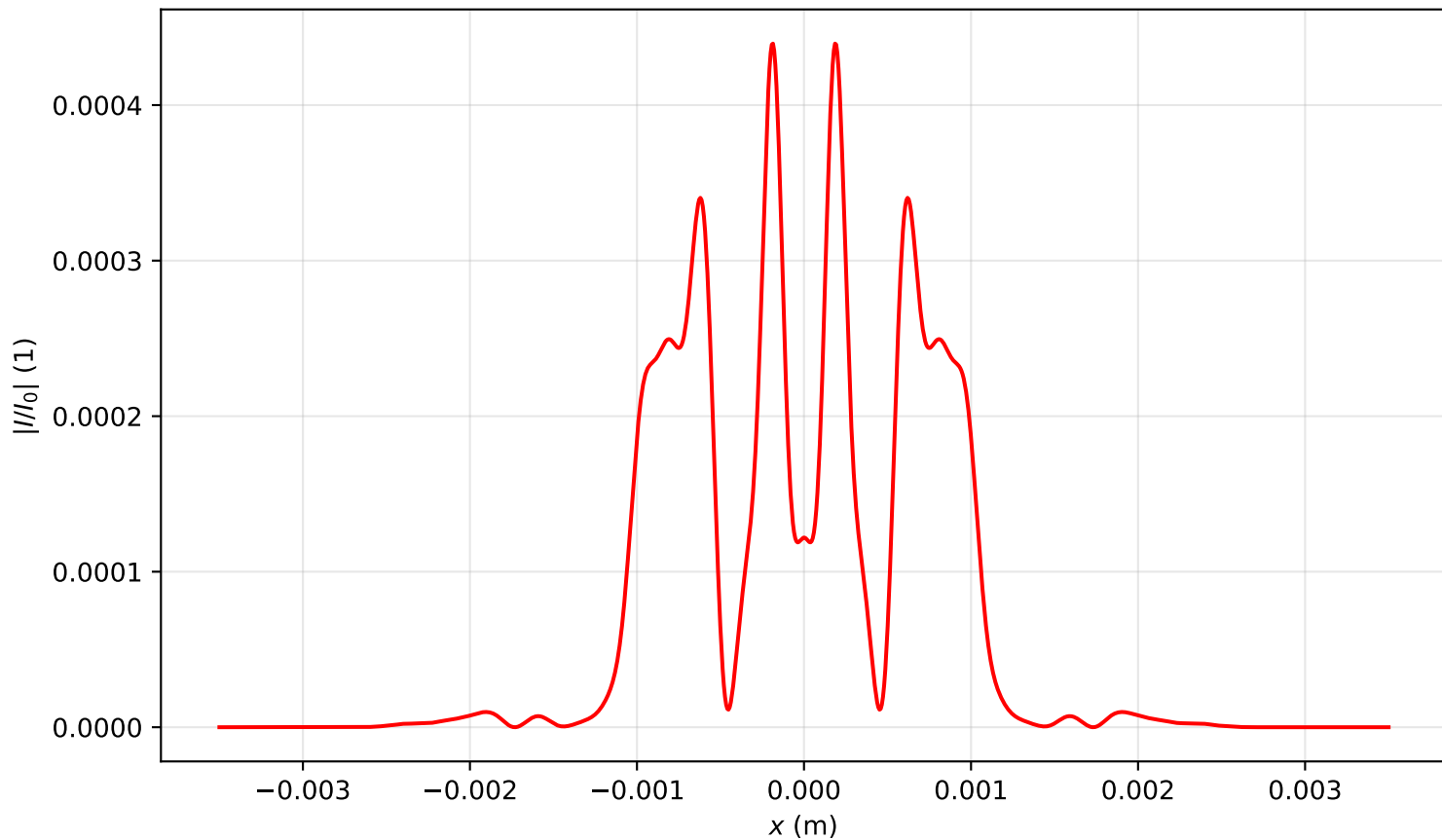
Intensity profile I(x, y = 0, z = 0.796)/I_0 , P_{in}=19.0P_{cr} , artificial time
