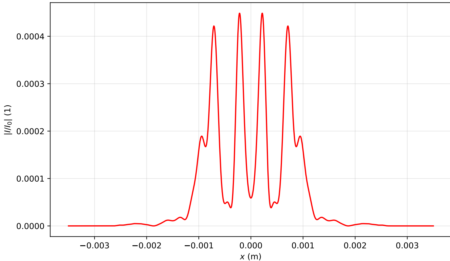
Intensity profile I(x, y = 0, z = 0.876)/I_0 , P_{in}=19.0P_{cr} , artificial time
