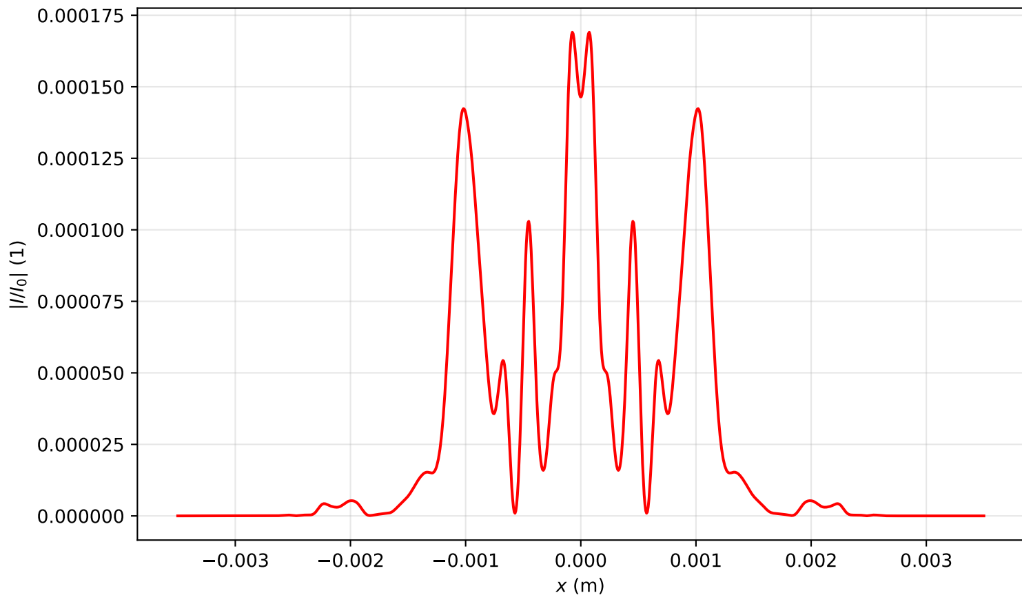
Intensity profile I(x, y = 0, z = 1.115)/I_0 , P_{in}=19.0\text{Pcr} , artificial time
