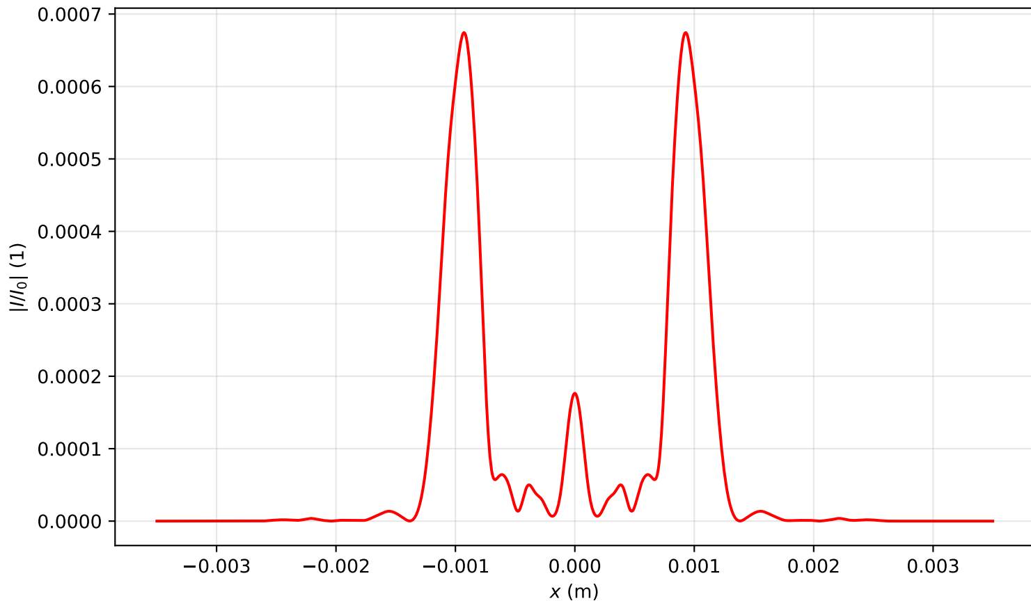
Intensity profile I(x, y = 0, z = 1.194)/I_0 , P_{in}=19.0\text{Pcr} , artificial time
