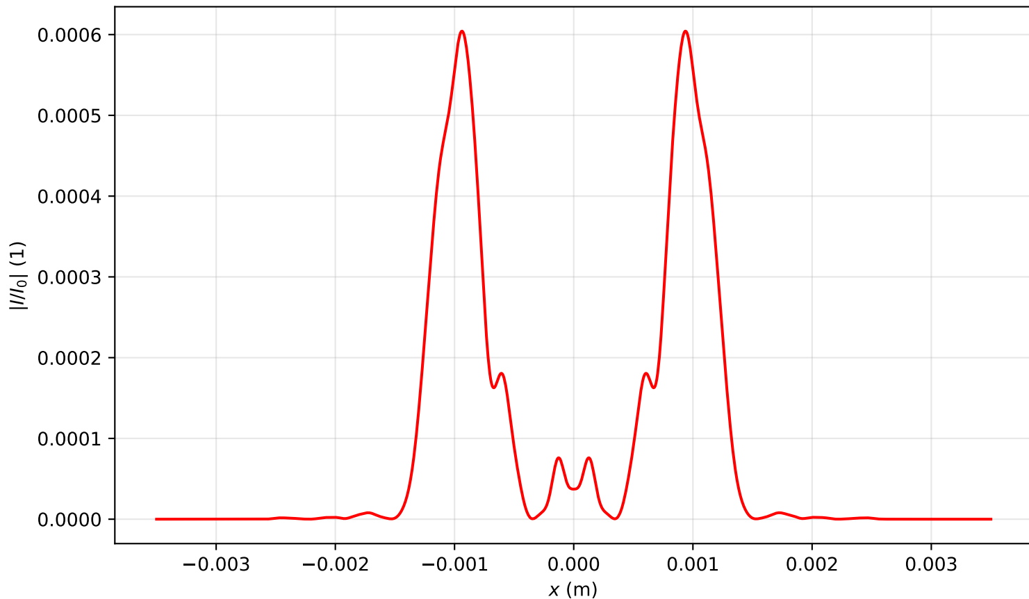
Intensity profile I(x, y = 0, z = 1.274)/I_0 , P_{in}=19.0\text{Pcr} , artificial time
