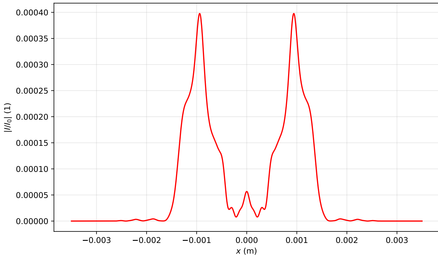
Intensity profile I(x, y = 0, z = 1.353)/I_0 , P_{in}=19.0P_{cr} , artificial time
