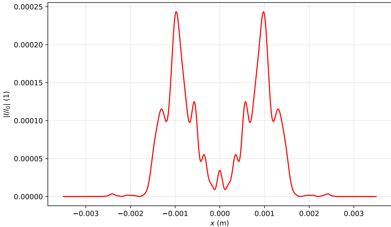
Intensity profile I(x, y = 0, z = 1.433)/I_0 , P_{in}=19.0P_{cr} , artificial time
