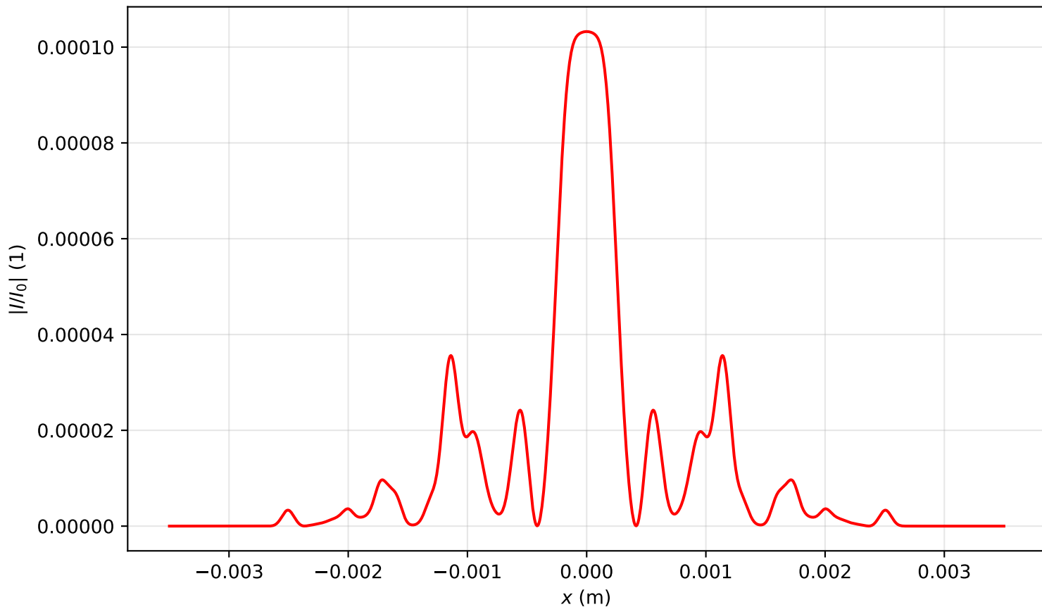
Intensity profile I(x, y = 0, z = 1.831)/I_0 , P_{in}=19.0P_{cr} , artificial time
