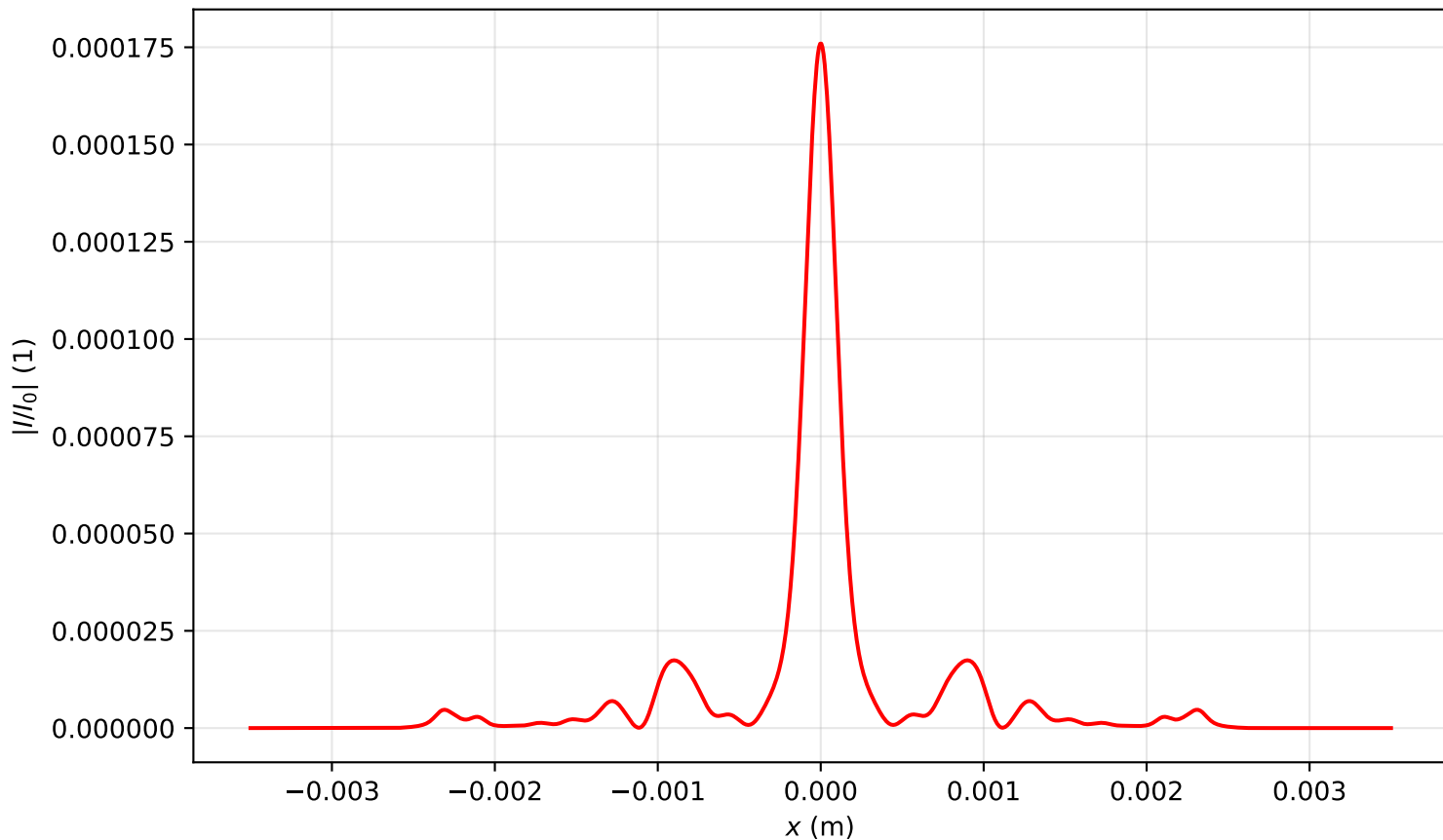
Intensity profile I(x, y = 0, z = 1.990)/I_0 , P_{in}=19.0\text{Pcr} , artificial time
