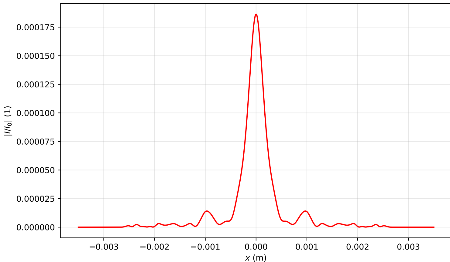
Intensity profile I(x, y = 0, z = 2.070)/I_0 , P_{in}=19.0\text{Pcr} , artificial time
