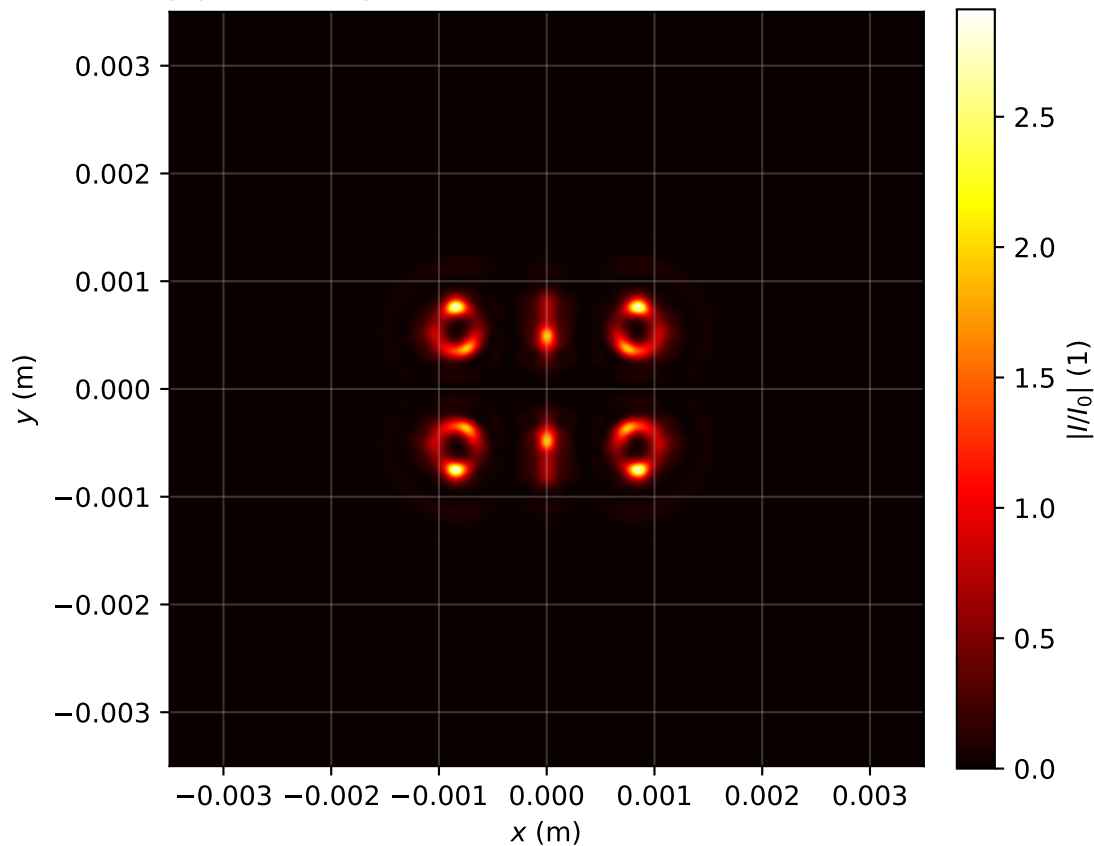
Intensity profile I(x, y, z = 0.478)/I_0 , P_{in}=19.0\text{Pcr} , artificial time
