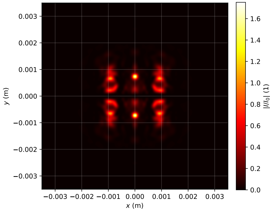
Intensity profile I(x, y, z = 1.115)/I_0 , P_{in}=19.0\text{Pcr} , artificial time
