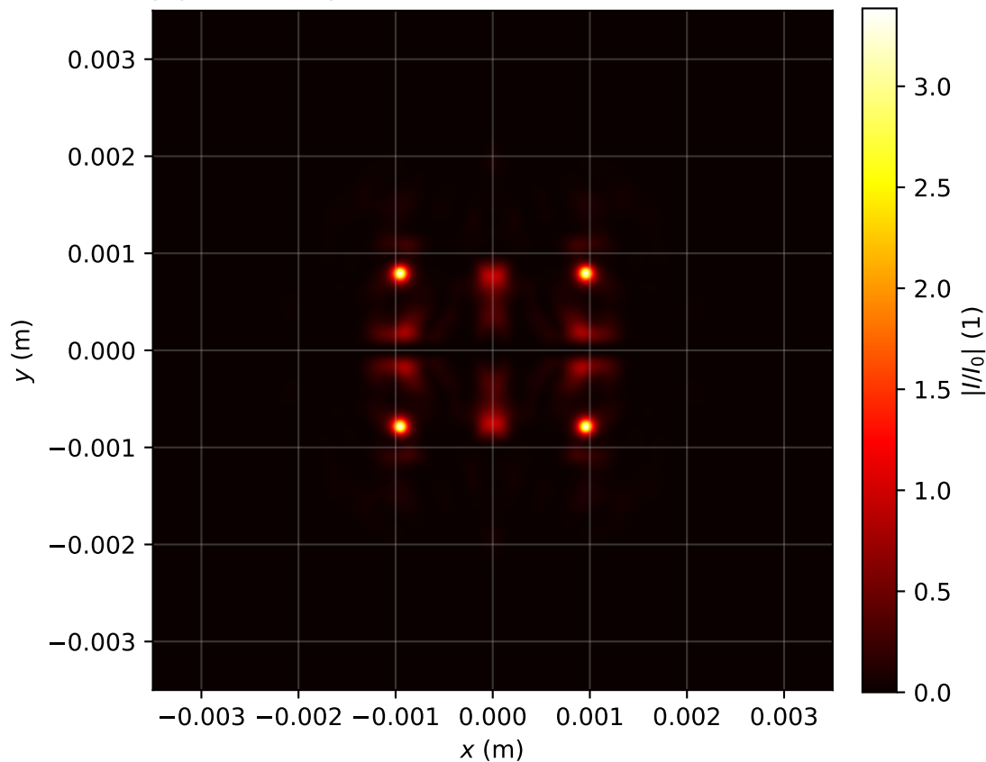
Intensity profile I(x, y, z = 1.274)/I_0 , P_{in}=19.0\text{Pcr} , artificial time
