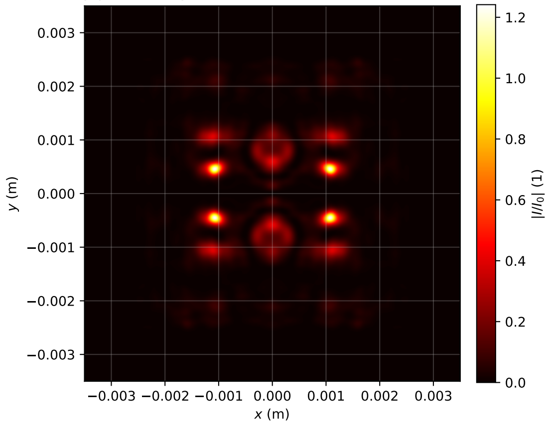
Intensity profile I(x, y, z = 1.990)/I_0 , P_{in}=19.0\text{Pcr} , artificial time
