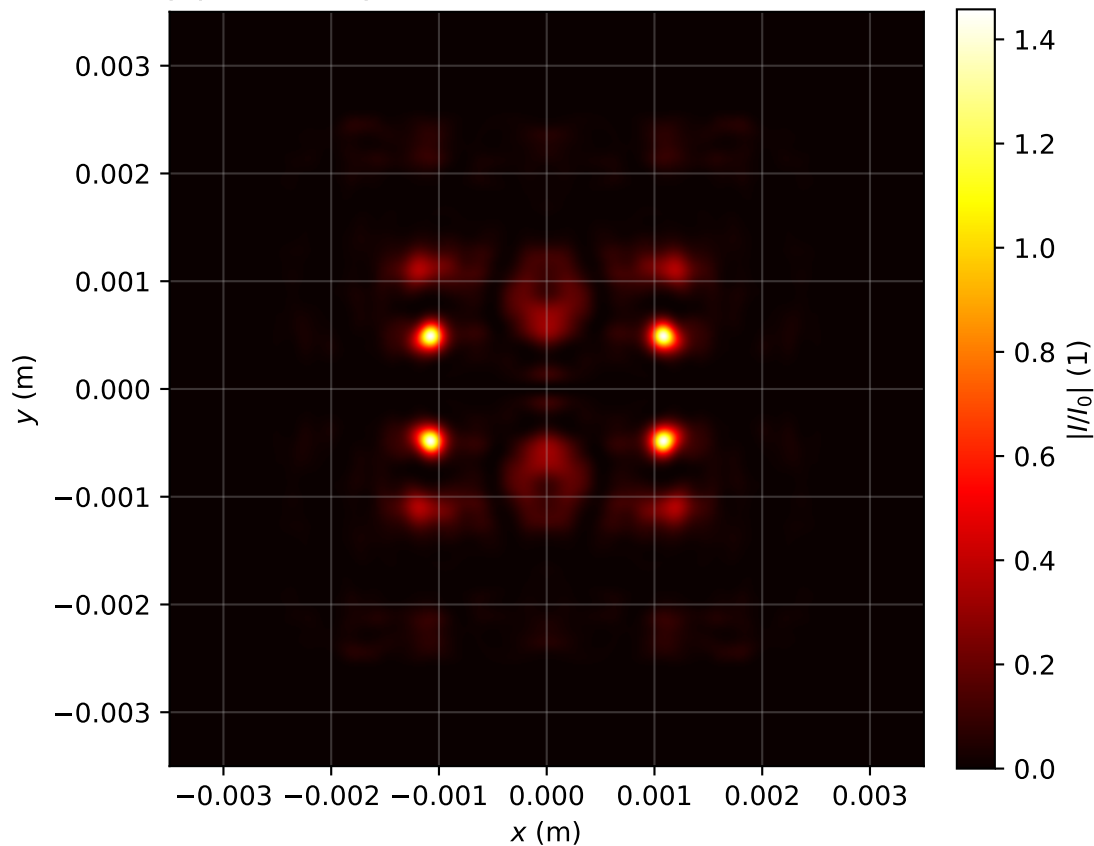
Intensity profile I(x, y, z = 2.070)/I_0 , P_{in}=19.0\text{Pcr} , artificial time
