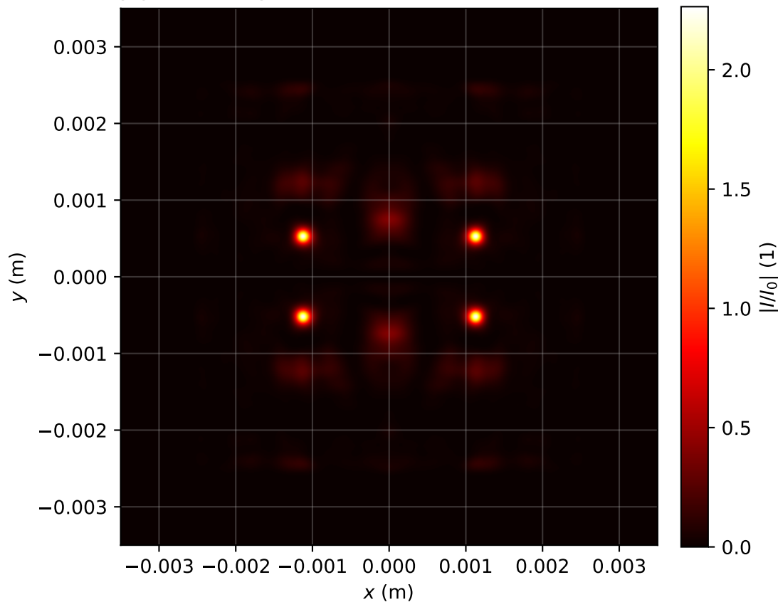
Intensity profile I(x, y, z = 2.229)/I_0 , P_{in}=19.0\text{Pcr} , artificial time
