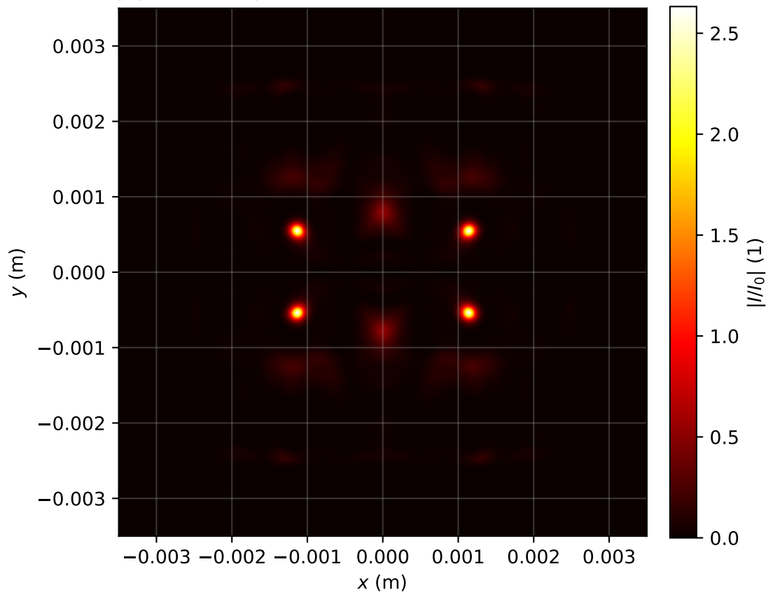
Intensity profile I(x, y, z = 2.309)/I_0 , P_{in}=19.0\text{Pcr} , artificial time
