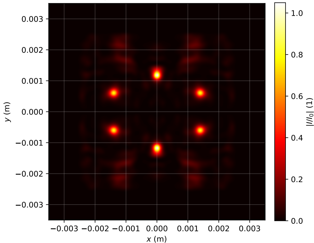
Intensity profile I(x, y, z = 3.344)/I_0 , P_{in}=19.0P_{cr} , artificial time
