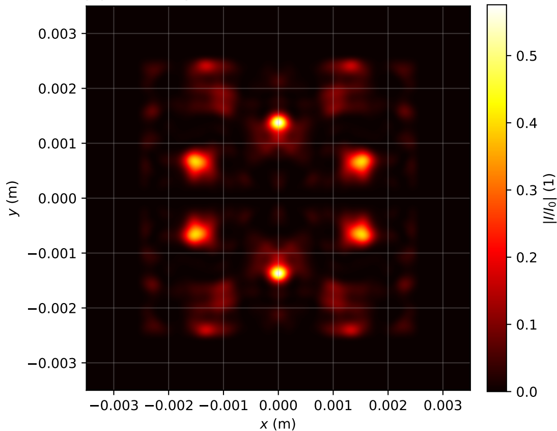
Intensity profile I(x, y, z = 3.582)/I_0 , P_{in}=19.0\text{Pcr} , artificial time
