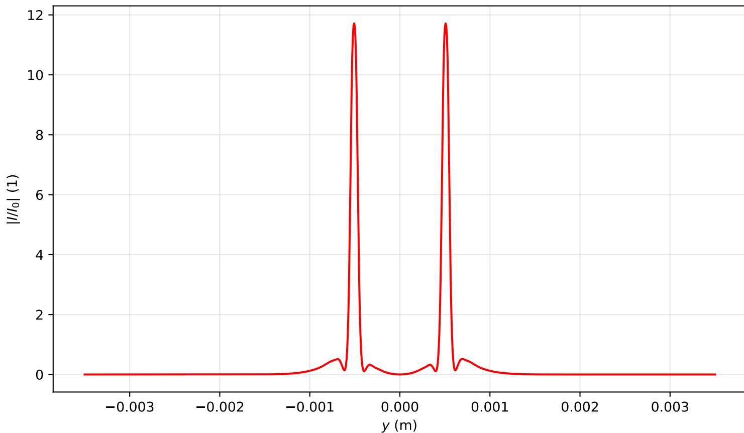
Intensity profile I(x=0, y, z=0.318)/I_0 , Pin=19.0Pcr, artificial time
