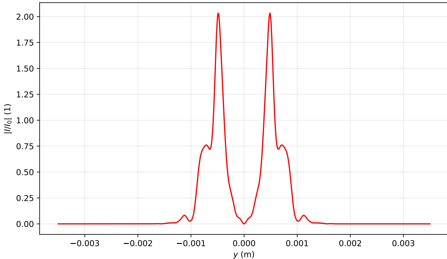
Intensity profile I(x=0, y, z=0.478)/I_0 , P_{in}=19.0P_{cr} , artificial time
