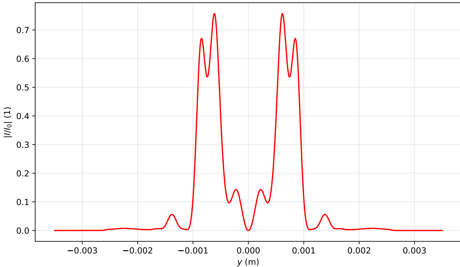
Intensity profile I(x=0, y, z=0.955)/I_0 , P_{in}=19.0\text{Pcr} , artificial time
