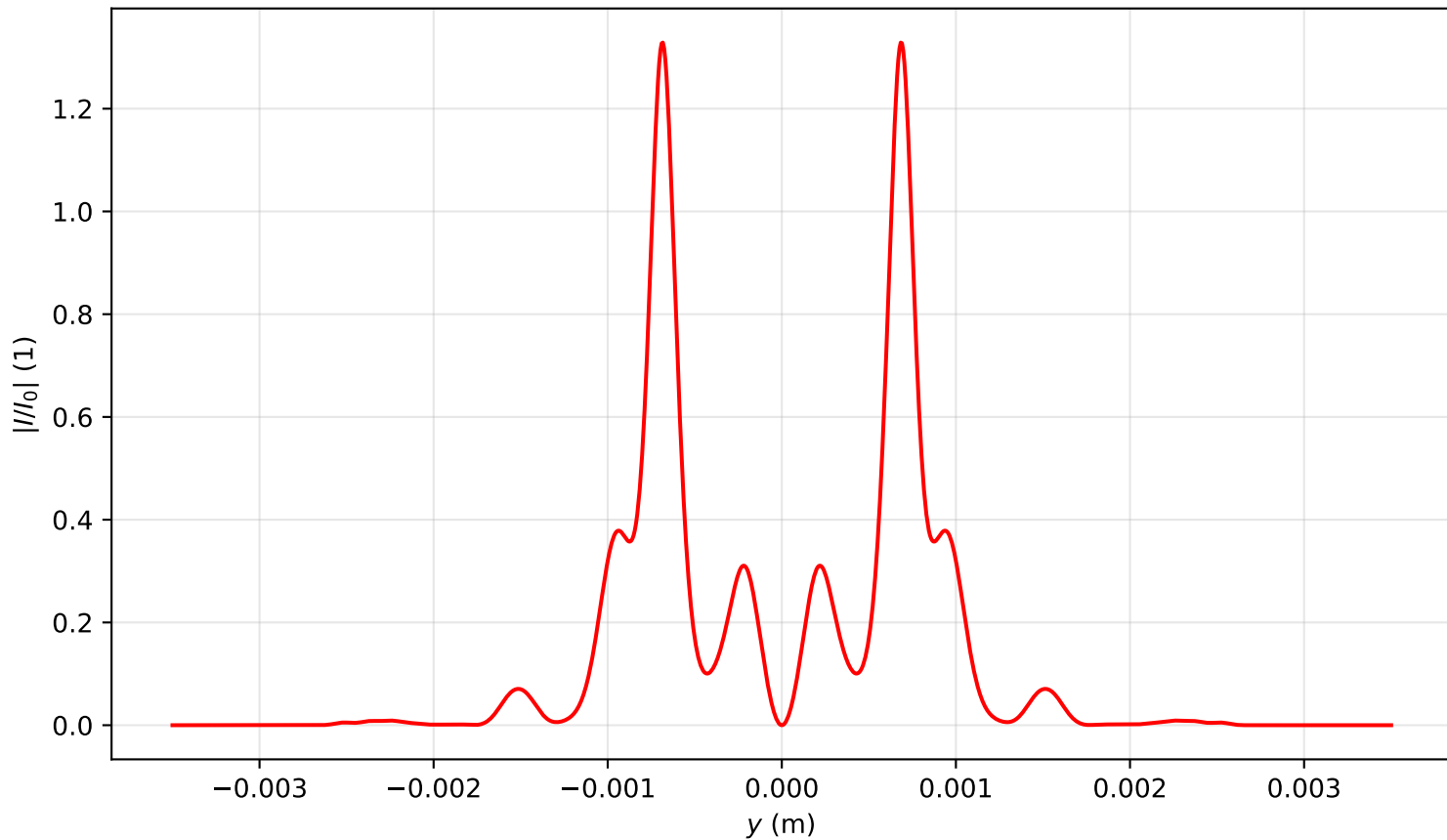
Intensity profile I(x=0, y, z=1.035)/I_0 , P_{in}=19.0P_{cr} , artificial time
