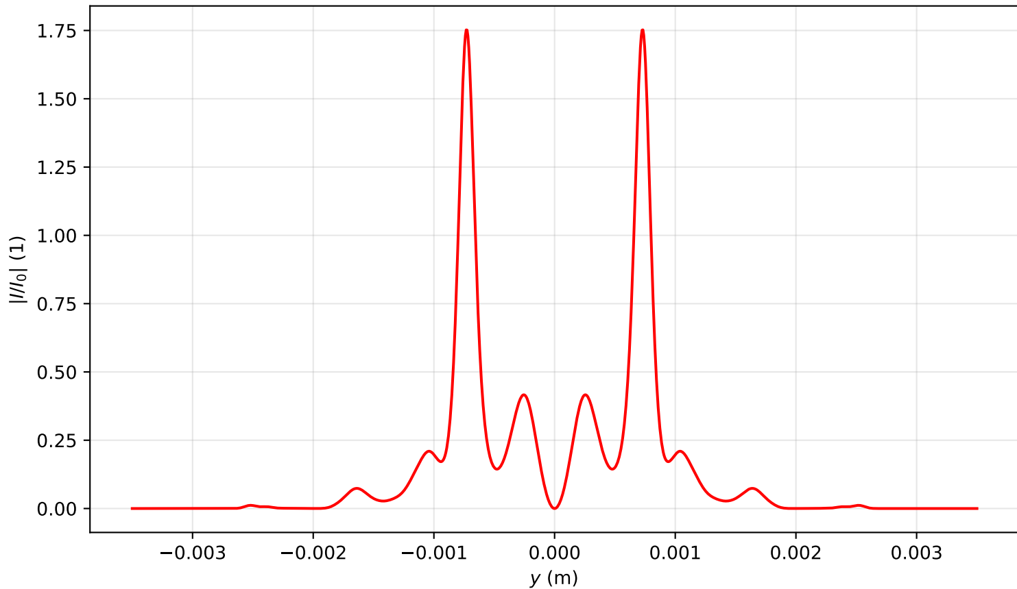
Intensity profile I(x=0, y, z=1.115)/I_0 , P_{in}=19.0\text{Pcr} , artificial time
